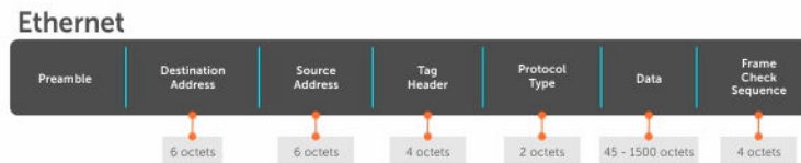
Figure 117. Tagged Frame Format
